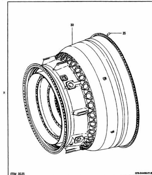
CORE MODULE-MAJOR ASSEMBLIES FIGURE 1 - SHEET 2
